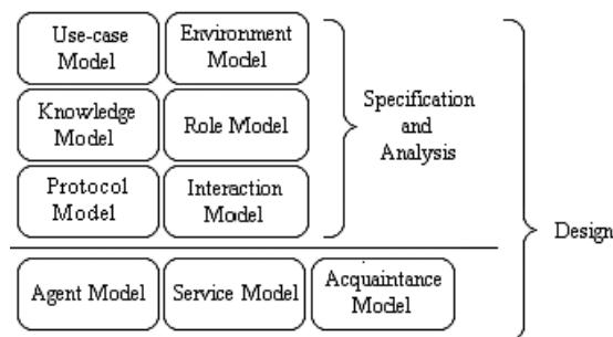
Fig. 2. Overview of ROADMAP
