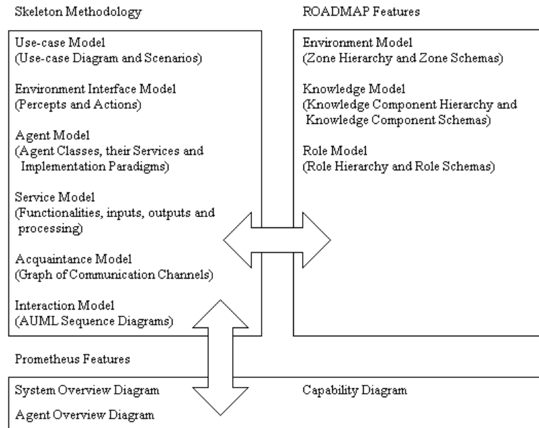
Fig. 3. Overview of the skeleton methodology and optional features from Prometheus and ROADMAP
