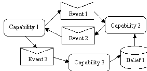
Fig. 9. Example Agent Overview Diagram
