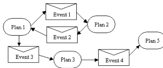
Fig. 10. Example Capability Overview Diagram
