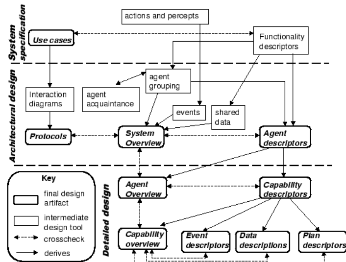
Fig. 1. Overview of 3 Phases in Prometheus
