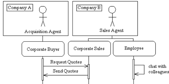
Fig. 7. An Example of Interaction Diagram with Roles and Zones
