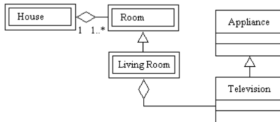
Fig. 5. An example of Zone Hierarchy with Objects
